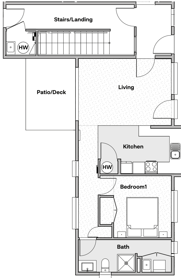
FLOOR PLAN
